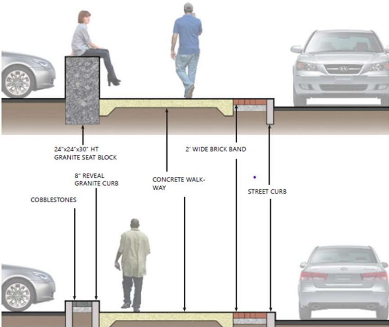
2' Wide Pedestrian Buffers
