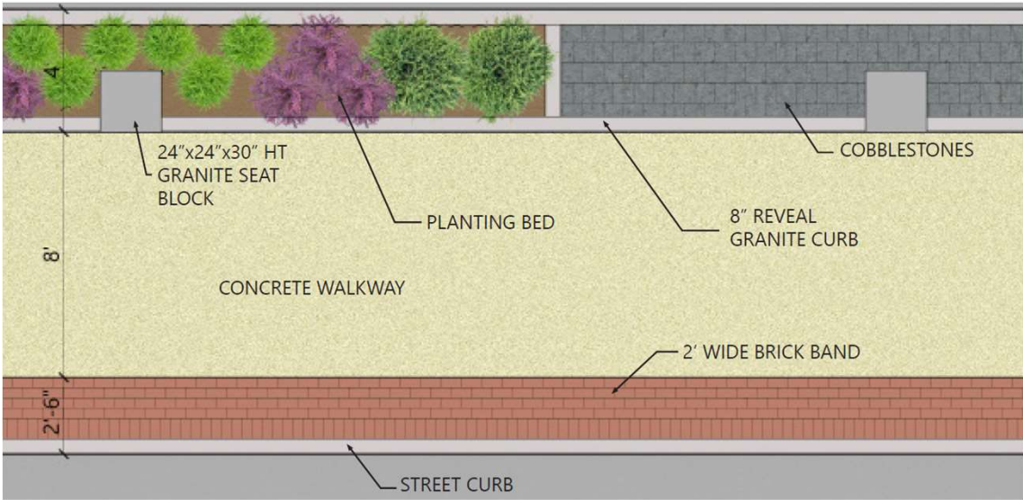
4' Wide Pedestrian Buffers
