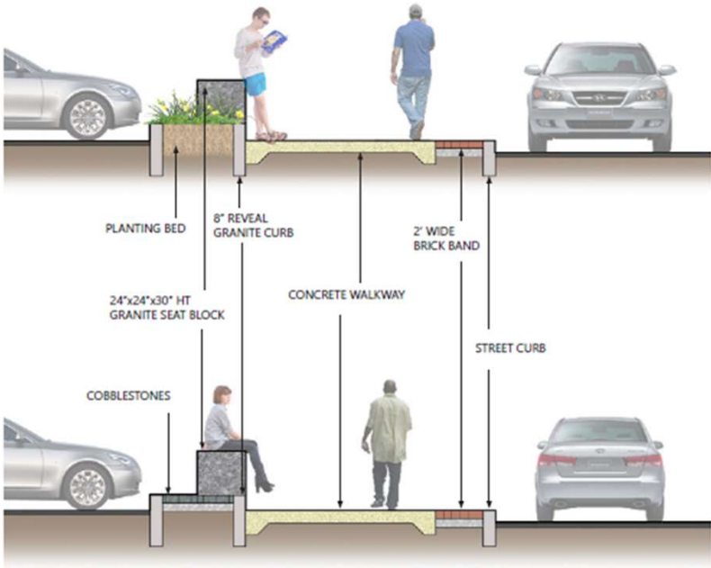
4' Wide Pedestrian Buffers
