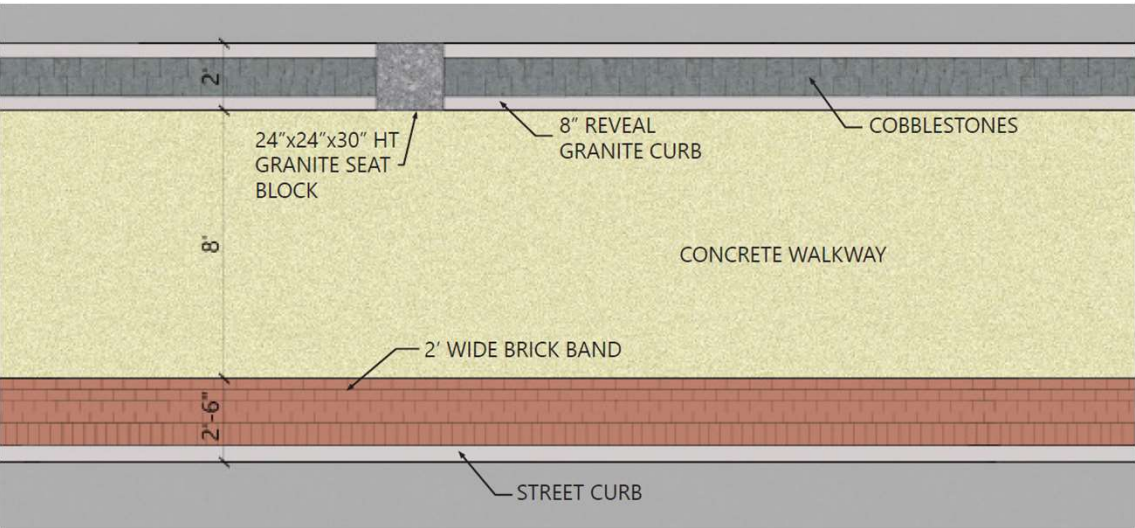
2' Wide Pedestrian Buffers
